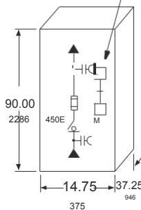
5 kV Indoor N1 top cable in/bottom cable out switch in position B
