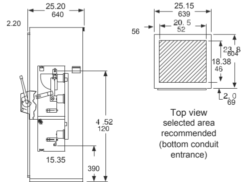
Section view (fused)
