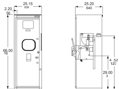
Section view (unfused)
